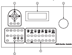
Front Panel Layout
